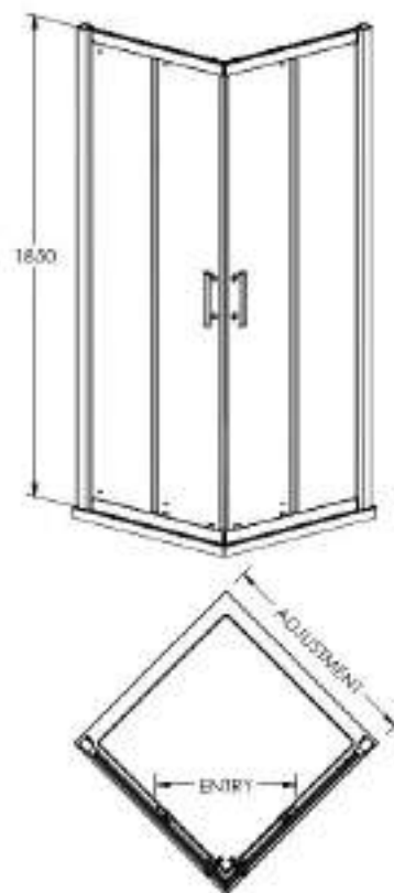
Pacific Corner Entry Enclosure
