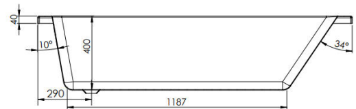
SECTION F-F SCALE 1 : 10
