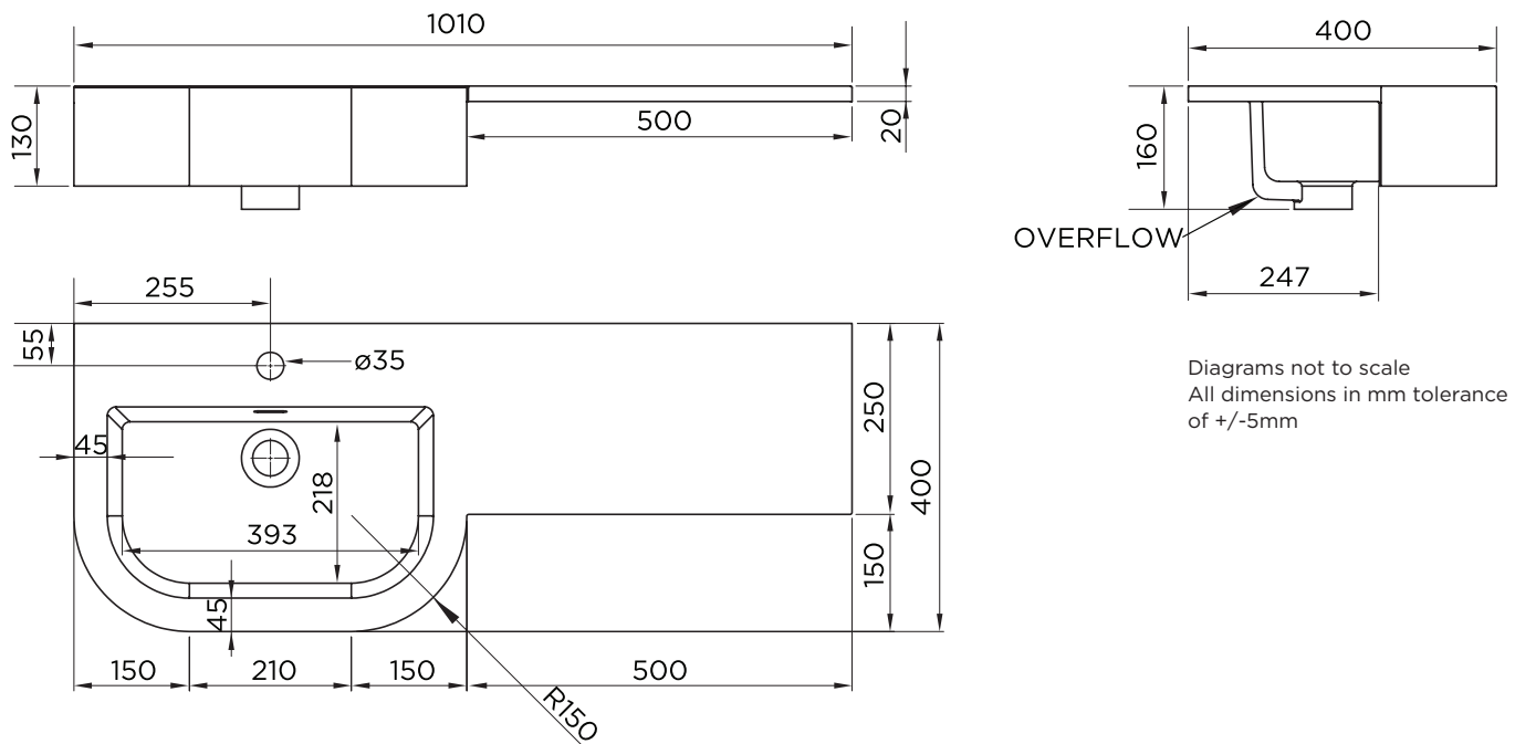
Left Hand basin shown
