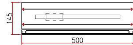
Vertical View
