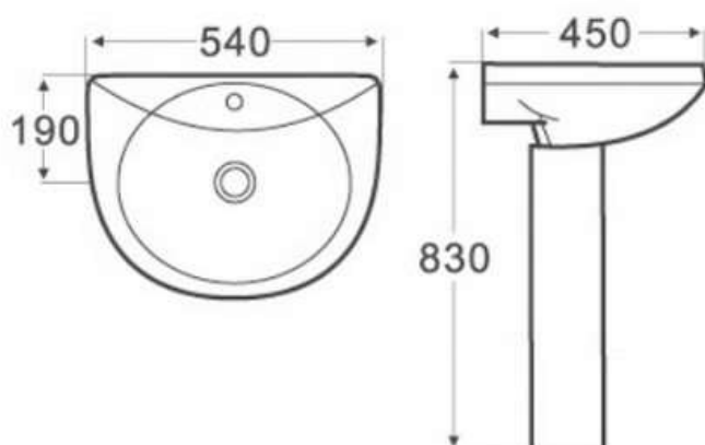
Pedestal Basin Size: 540x450x830mm Fixing to wall with back
