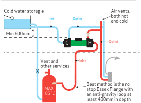
Figure 7: Typical Right Pump Installation - pump located above the cylinder
