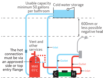
Figure 6: Typical Right Pump Installation - pump located at base of the cylinder
