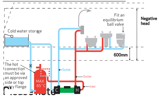
Figure 8: Negative head
