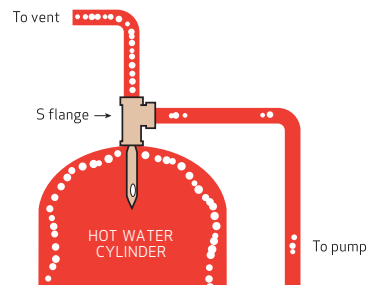
Figure 22: S flange
