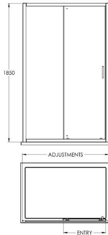
SQ Slider Enclosure
