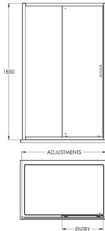
SQ Slider Enclosure
