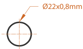
A SECTION
