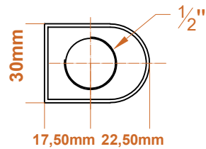
B SECTION
