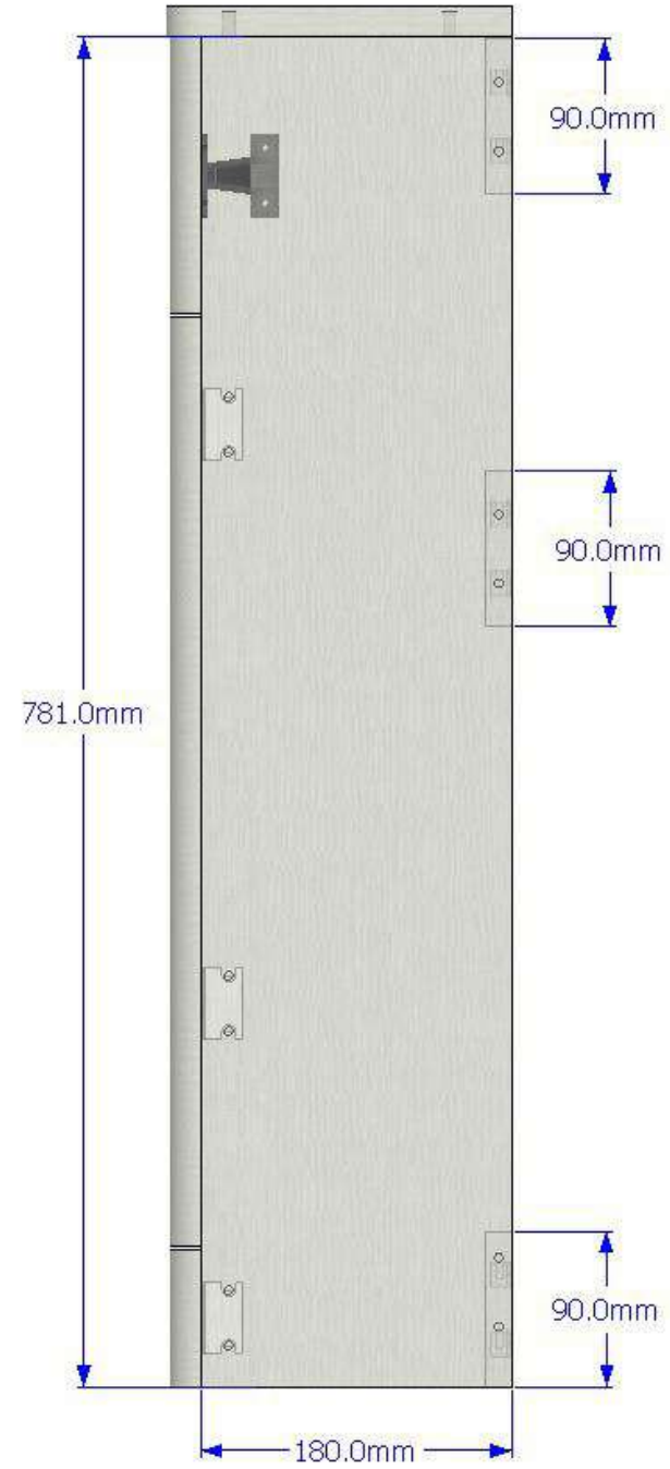
WC - End Elevation
