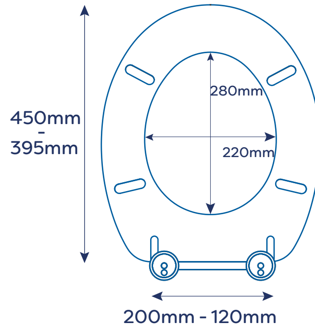
Max/Min Adjustment
